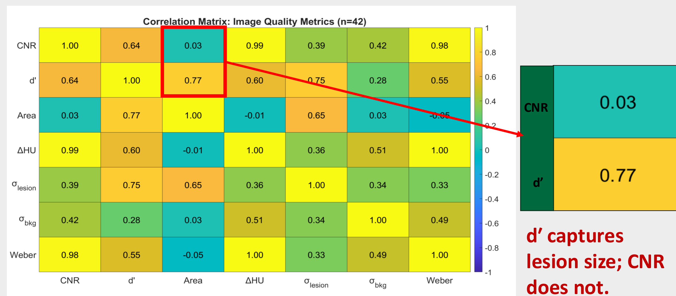
Figure 2. Pearson correlation heatmap of image quality metrics (n=42). CNR correlates near-perfectly with lesion contrast (ΔHU: r=0.99) and Weber contrast (r=0.98) but not with lesion area (r=0.03). Detectability index (d') correlates with both area (r=0.77) and contrast (r=0.60), capturing geometric factors CNR misses. Color scale: -1 (blue) to +1 (yellow).
