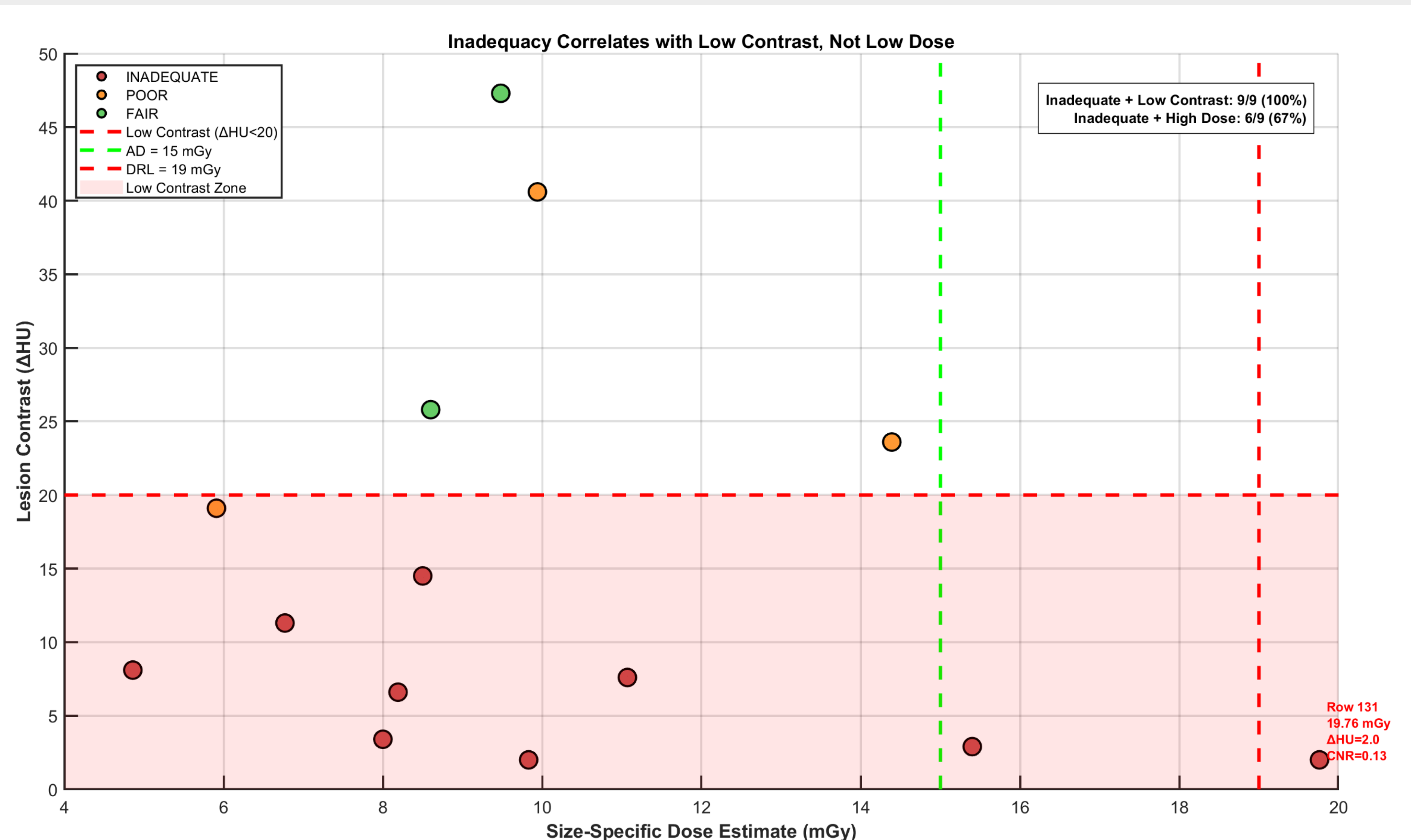
Figure 3. Lesion contrast (ΔHU) vs. SSDE for all assessed cases, stratified by IQ adequacy. 100% of IQ-inadequate cases (red zone) fell below ΔHU = 20 , while 67% occurred at doses above 8 mGy — confirming that low contrast, not low dose, drives detectability failure. The extreme case at 19.76 mGy with CNR = 0.13 (above the ACR DRL yet non-diagnostic) demonstrates that dose escalation cannot rescue insufficient lesion contrast. Vertical and horizontal reference lines mark the contrast and dose thresholds, respectively.
