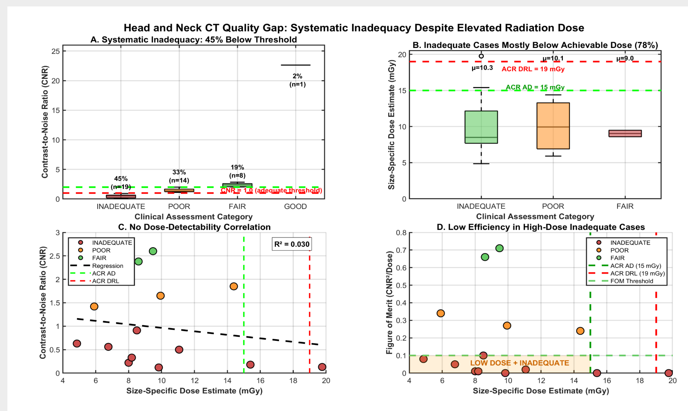
Figure 1A-D: Systematic quality gap analysis in clinical neck CT (n=42). (A) CNR distribution shows 45% inadequacy. (B) IQ-Inadequate cases at elevated dose (μ=10.3±4.6 mGy vs 9.7±3.1 mGy adequate). (C) No dose-detectability correlation (R 2 =0.030). (D) Low dose efficiency (FOM) in high-dose IQ-inadequate cases ("waste zone").
